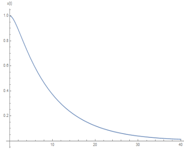
Figure 1: An overdamped harmonic oscillator approaching equilibrium slowly.
