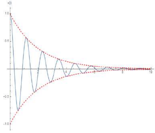
Figure 2: Underdamped oscillations within an exponential decay envelope.
